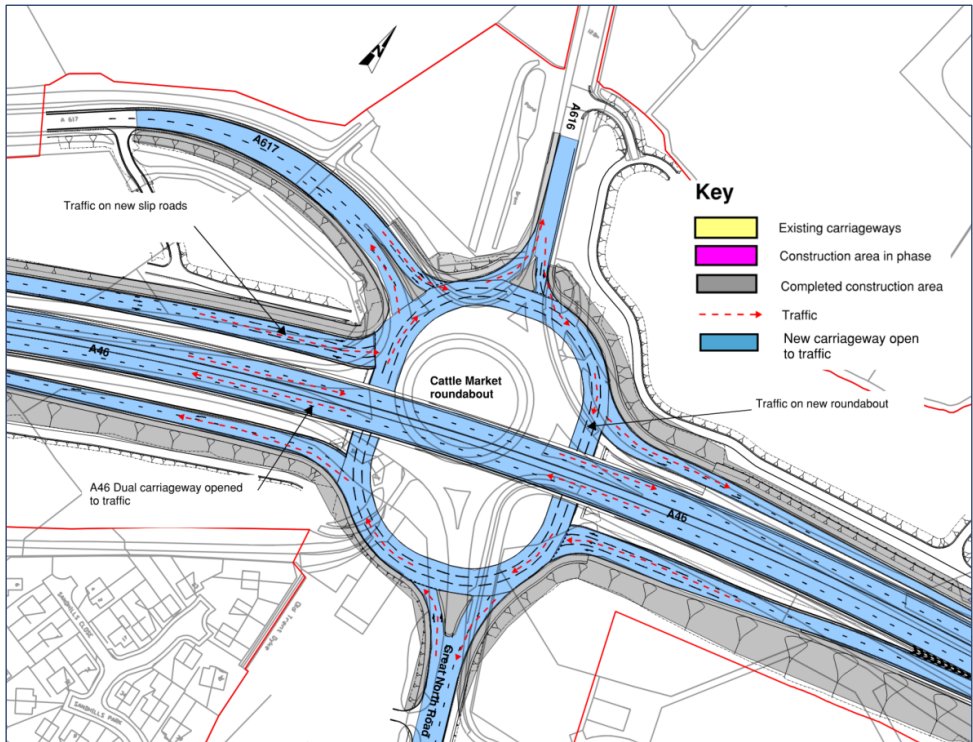
Appendix Figure A-12: Cattle Market Junction Construction Phase 5
