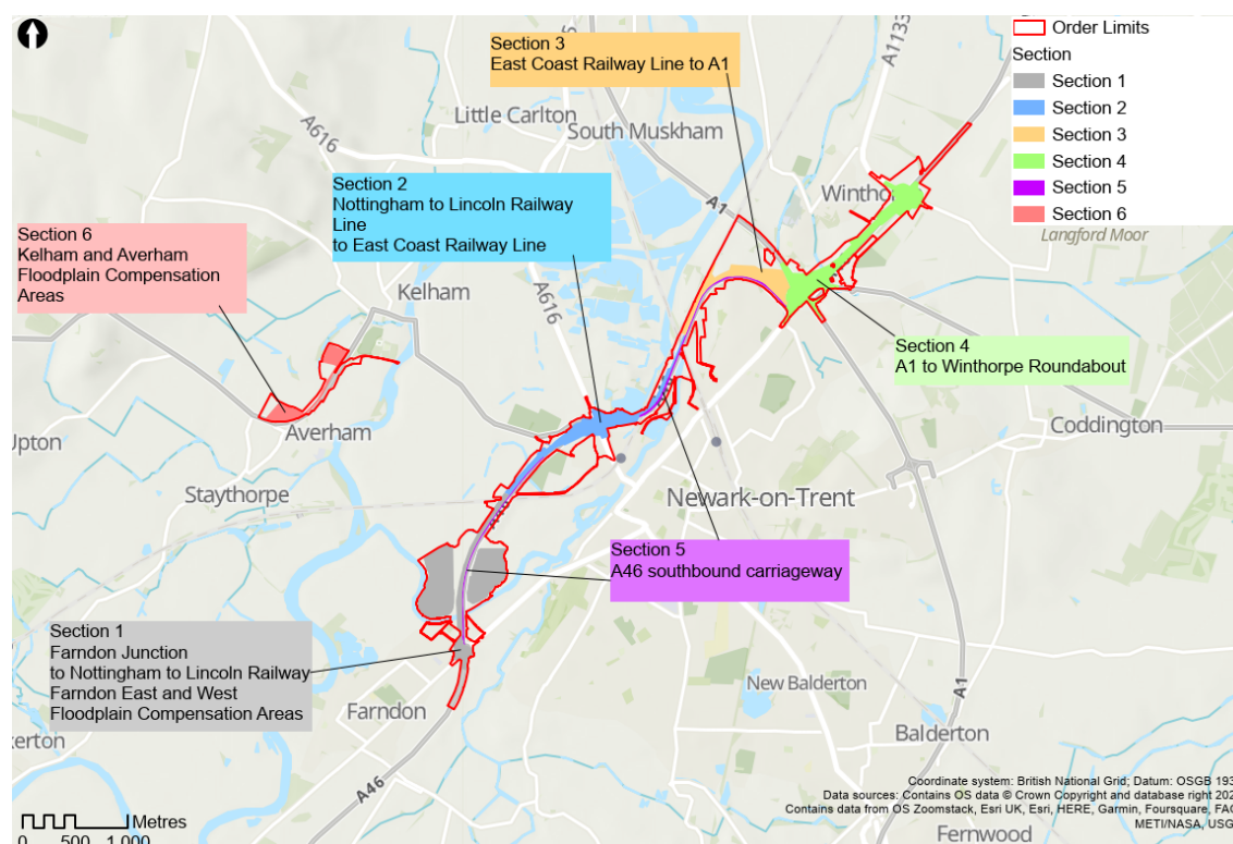
Figure 2-1: Main construction works sections
